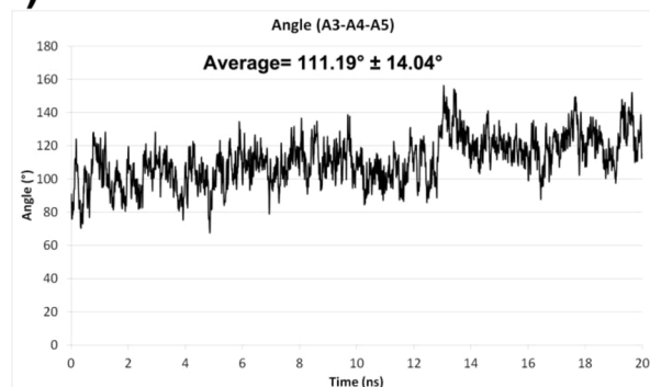
Figure 5. (a) Front view of the average M1 structure deriving from the 20 ns MD production run together with a pictorial representation of its sugar residue sequence. Repetitions 1, 2, 3, 4, and 5 are represented as blue, red, green, yellow, and magenta sticks, respectively. The C2 atoms of the A1–A6 sugar residues, used to calculate the hinge angles are represented as spheres. Plots of the hinge angle values (deg) formed by the C2 atoms of the A1–A2–A3, A2–A3–A4, A3–A4–A5, and A4–A5–A6 are represented in (b), (c), (d), and (e), respectively. The degree of flexibility for each hinge angle is calculated as the standard deviation from the values obtained from the last 20 ns of simulation.
